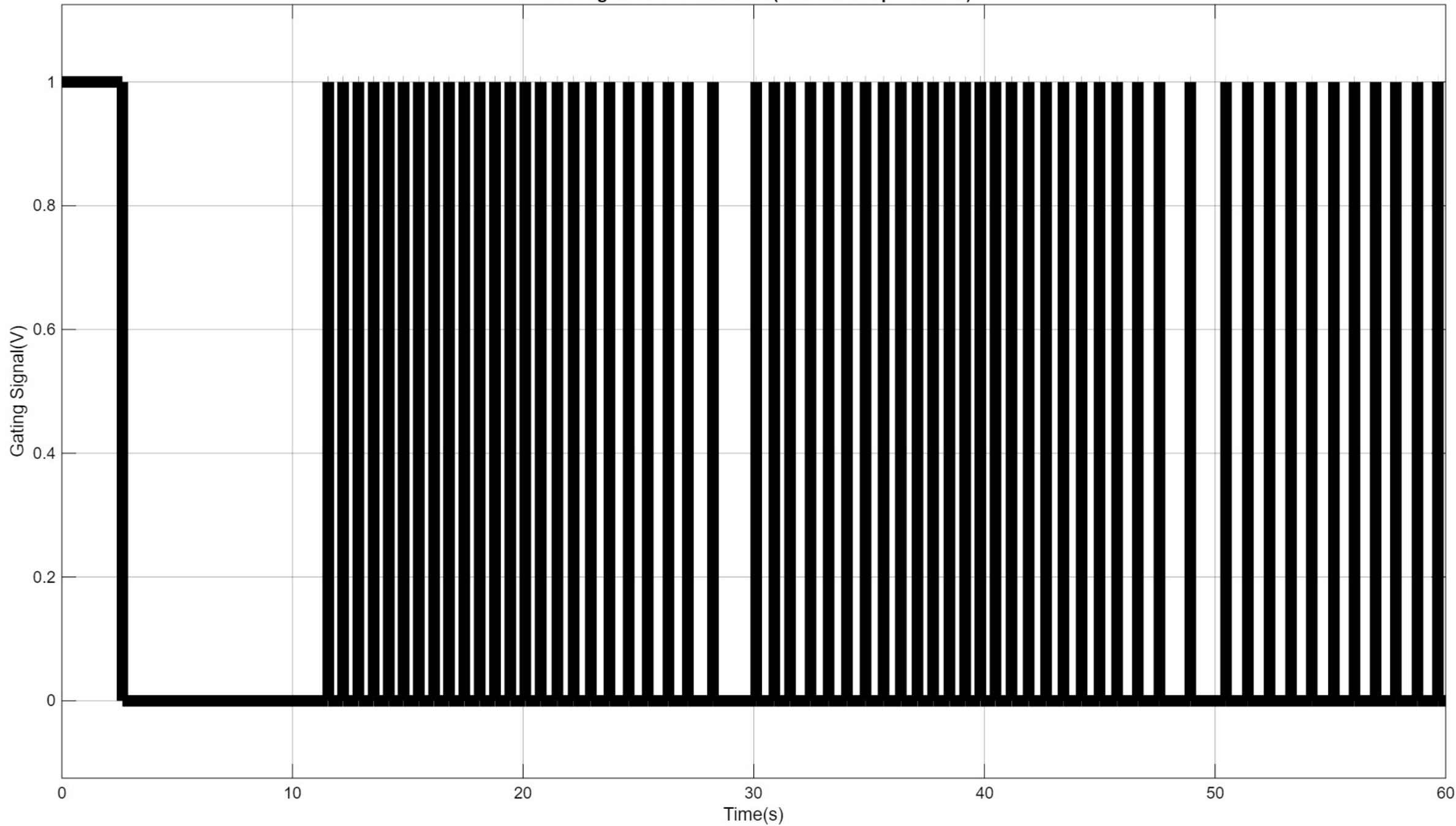
Gate Signal of Buck Mosfet ( Closed Loop Control )
